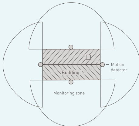
Comprehensive monitoring zone made up of four eNet motion detectors
